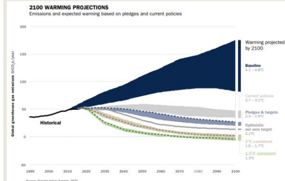
Figure: Global Greenhouse Gas (GHG) emissions GtCO 2 e/year
